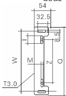
柜外操作安装底板尺寸 the cabinet outside base installation dimensions
