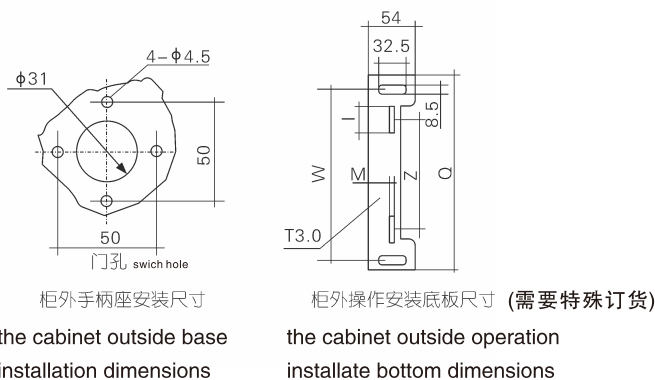
GSG2-160~630 inside the cabinet operating
