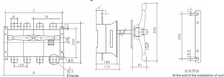
GSG2-1600/JH柜外操作 GSG2-1600/JH the cabinet outside operation
