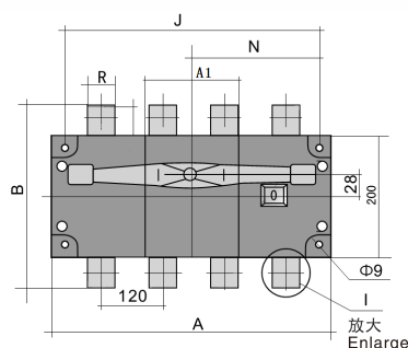
GSG2-1600/J柜外操作 GSG2-1600/J the cabinet outside operation
