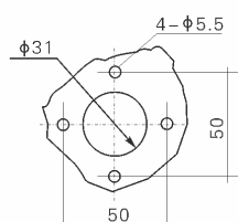
柜外手柄座安装尺寸 the cabinet outside base installation dimensions
