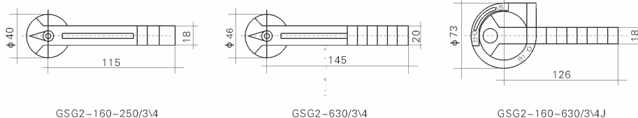
Picture1 GSG2-160~1600 Isolation Switches
