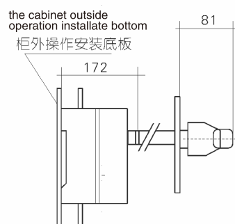
柜外操作安装底板尺寸 the cabinet outside operation installate bottom dimensions
